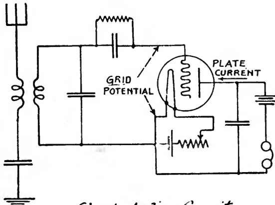
Simple Audion Circuit (de Forest Catalog C, page 30, with "Audion" Connection)
